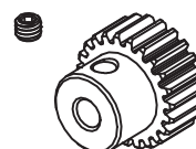
24T Pinion Gear, 48P
