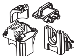
Central Differential Mount
